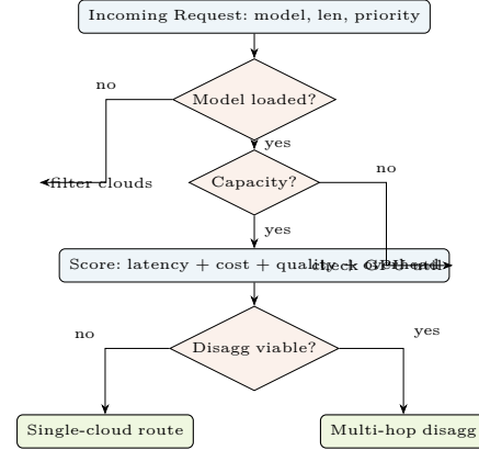
Fig. 8. Multi-objective routing decision framework. Each request is scored across latency, cost, quality, and overhead dimensions before selecting single-cloud or disaggregated multi-hop routing.
