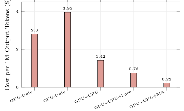
Fig. 4. Cost per million output tokens across deployment strategies (Llama-70B). GPU+CPU with speculative decoding and MemoryAlloy achieves $0.22/M, a 12.7× reduction vs. GPU-only ($2.80/M).
