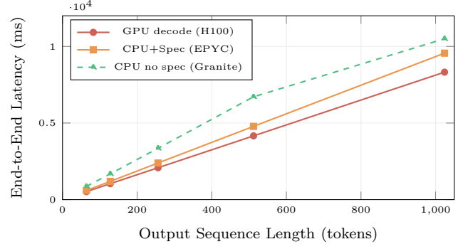
Fig. 5. End-to-end latency vs. output length. CPU+speculative decode tracks GPU within 15% up to 512 tokens. Beyond 512 tokens, the gap widens but remains within 2×. For 98% of production requests (<512 output tokens), CPU decode is latency-competitive.
