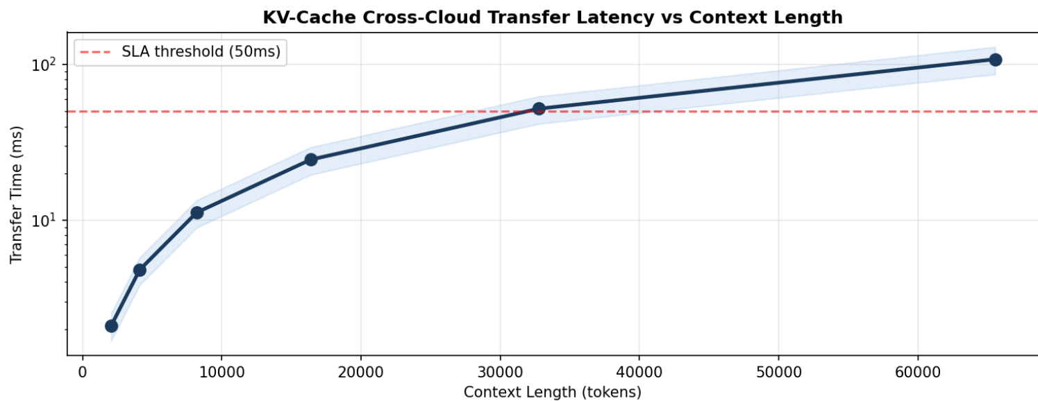
Figure 2. KV-cache transfer latency vs context length. SLA threshold breached at ~32K tokens, the practical boundary for cross-cloud disaggregation.
