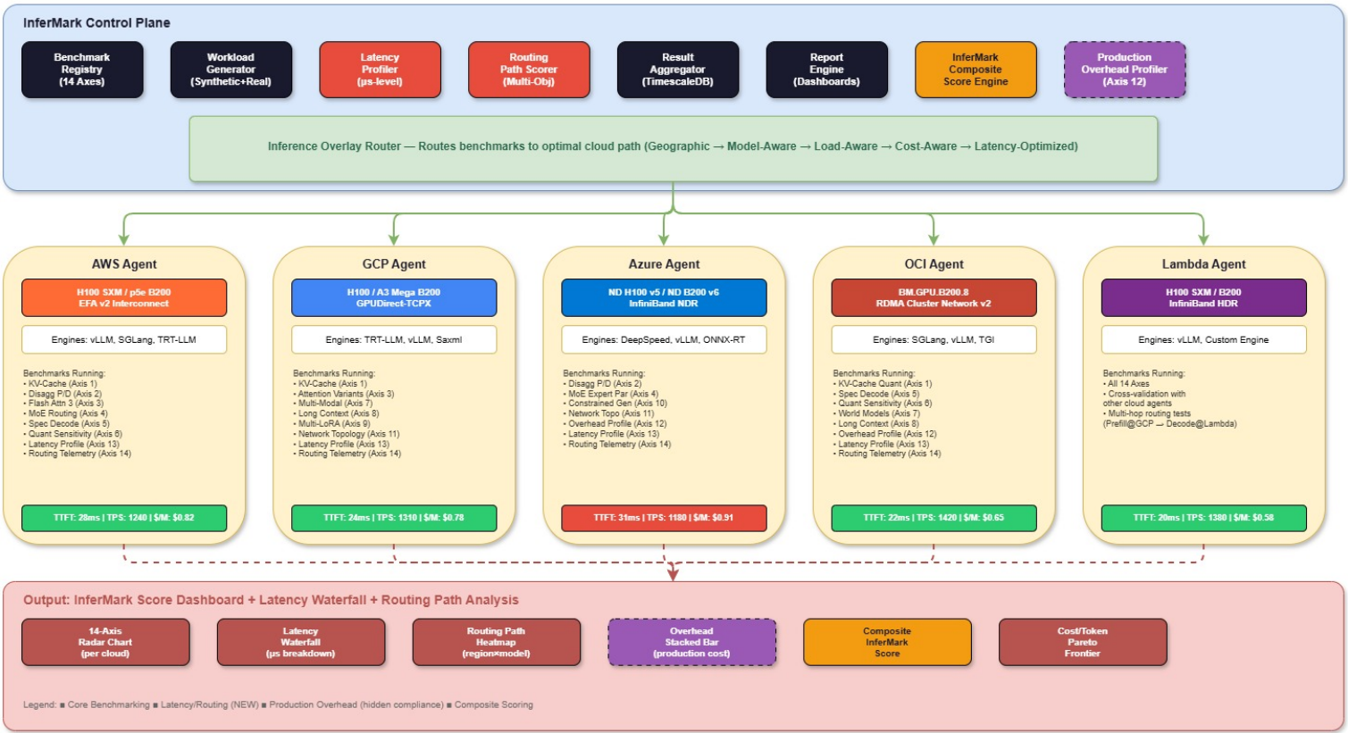
InferMark: 14-Axis Multi-Cloud Inference Benchmarking Platform
