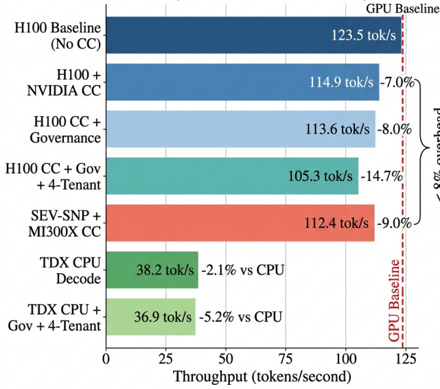
Fig. 5. Throughput comparison across confidential computing configurations. GPU baseline (123.5 tok/s) drops by only 7% with NVIDIA CC and 8% with full governance. CPU TDX decode operates at lower absolute throughput but with only 2.1–5.2% CC overhead. The <8% bracket highlights that confidential+governed GPU inference remains within acceptable production overhead.
