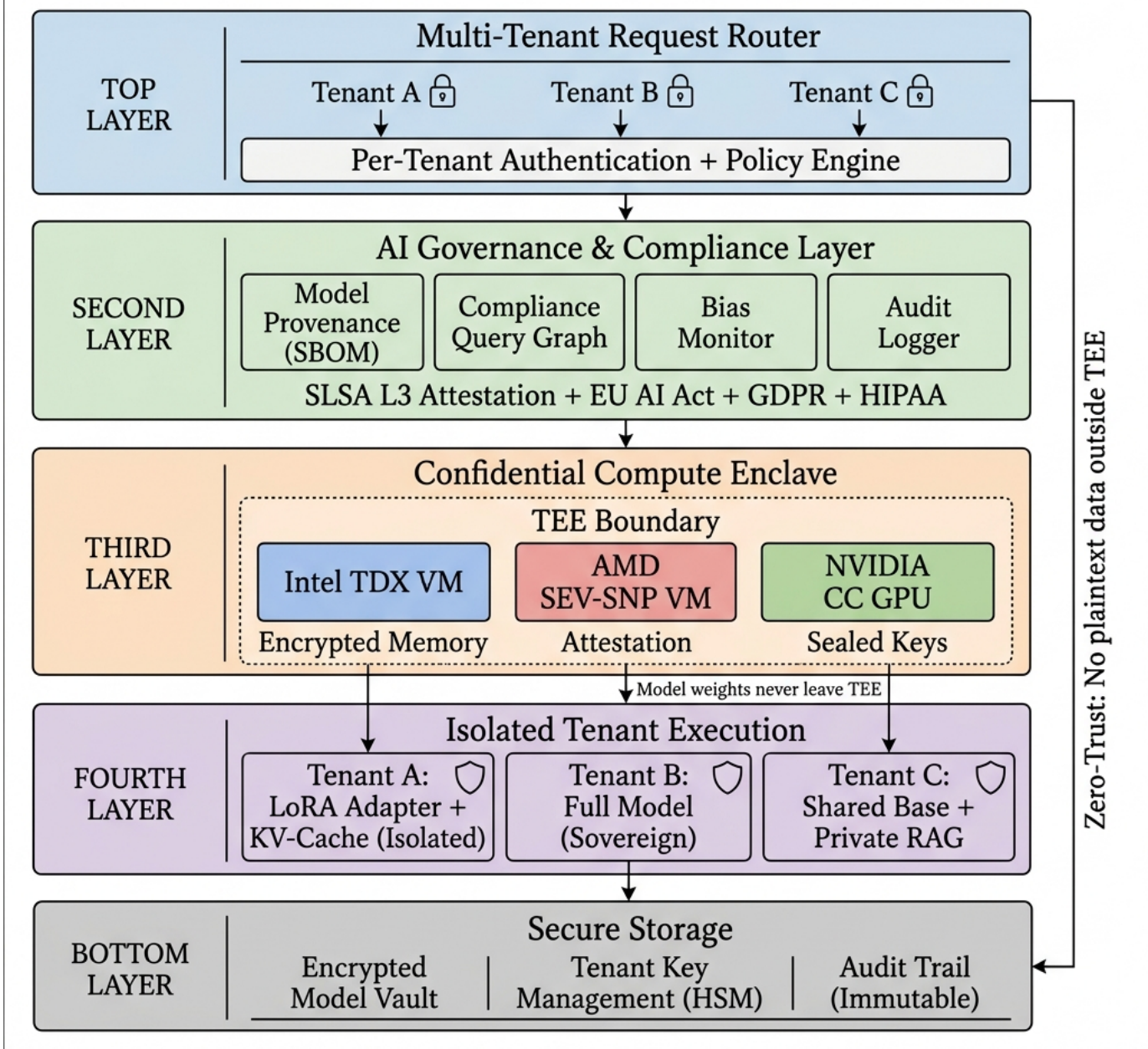
Fig. 1. Confidential multi-tenant LLM inference architecture. Layer 1: Multi-tenant request router with per-tenant authentication and policy enforcement. Layer 2: AI Governance and Compliance layer with SBOM provenance (Chainguard-style), compliance graph queries (Wiz-style), bias monitoring, and audit logging under SLISA L3, EU AI Act, GDPR, and HIPAA. Layer 3: Confidential compute enclave with TEE boundary spanning Intel TDX, AMD SEV-SNP, and NVIDIA CC GPU—model weights never leave the TEE. Layer 4: Isolated tenant execution with per-tenant LoRA adapters, sovereign full-model deployments, and shared-base with private RAG. Layer 5: Secure storage with encrypted model vault, HSM-backed key management, and immutable audit trail. Zero-trust principle: no plaintext data exists outside the TEE boundary.
