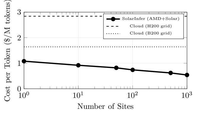
Fig. 8. Cost per million tokens vs. fleet scale. SolarInfer achieves sub-$0.55/M tokens at 1,000 sites due to volume procurement and operational leverage, 81% cheaper than H200 cloud.
