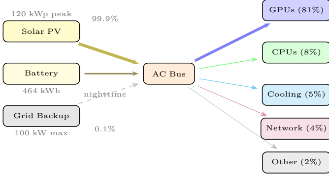
Fig. 4. Power distribution in the Edge SKU. Solar provides 99.9% of energy. GPUs consume 81% of total power. Grid backup is used <9 hours per year.
