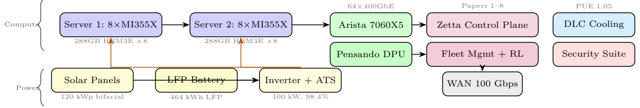
Fig. 2. SolarInfer Edge SKU complete architecture. Power tier (solar + BESS) feeds compute tier (2x8-GPU servers), connected via 400GbE fabric with DPU-based telemetry to the Zetta control plane. DLC cooling maintains PUE of 1.05.
