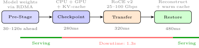
Fig. 4. CRIU migration pipeline. Pre-staging overlaps with active serving; user-visible downtime is only 1.3s for intra-vendor migration.
