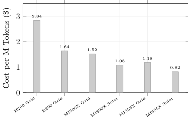
Fig. 3. Cost per million tokens across accelerator and power configurations. AMD MI355X with solar achieves $0.82/M tokens—71% cheaper than NVIDIA H200 on grid.
