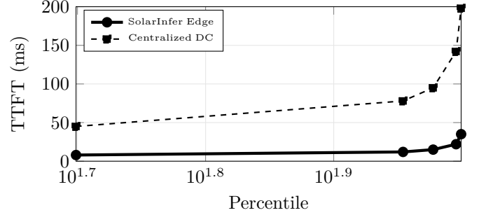
Fig. 4. Time-to-first-token latency: Edge (8ms P50) vs. centralized DC (45ms P50).
