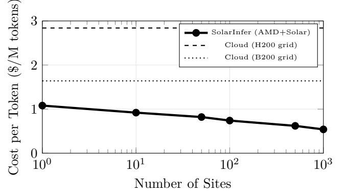
Fig. 6. Cost per million tokens vs. fleet scale. SolarInfer achieves sub-$0.55/M tokens at 1,000 sites due to volume procurement and operational leverage, 81% cheaper than H200 cloud.
