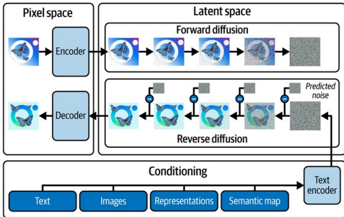
Figure 3-17. Stable Diffusion training and inference
