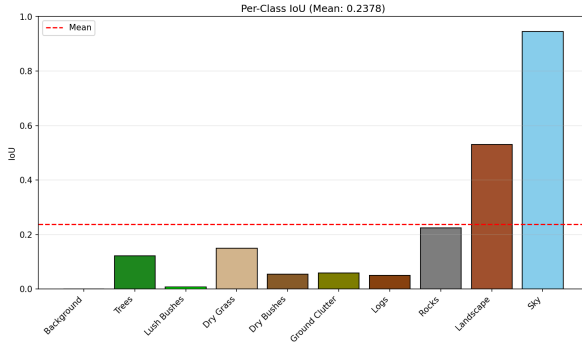
Figure 1: Baseline (v2) : Rare classes suppressed (mIoU 0.2378)
