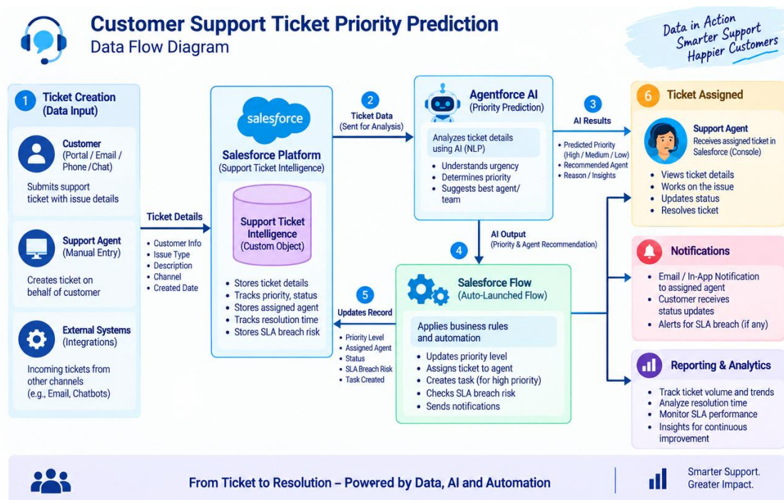
Figure 5: Data flow diagram for ticket priority prediction
