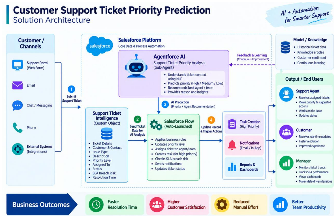
Figure 7: Solution architecture on the Salesforce platform
