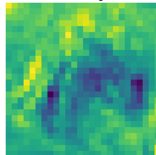
7x7 - map 4
