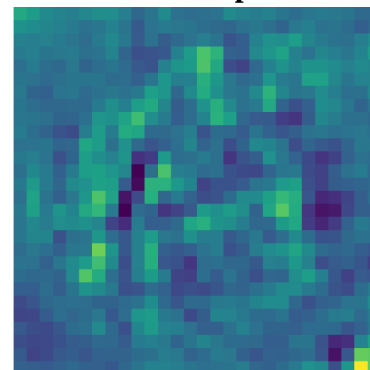
5x5 - map 4
