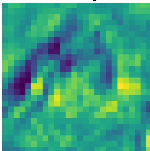
7x7 - map 2
