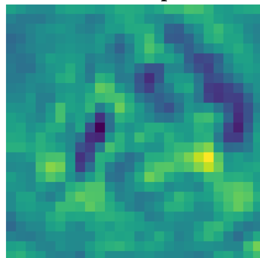
7x7 - map 1
