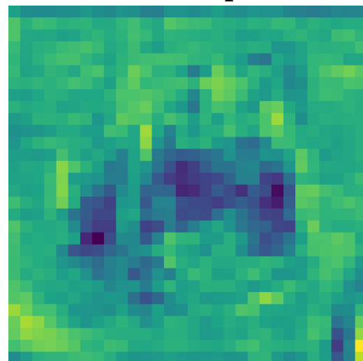
5x5 - map 1
