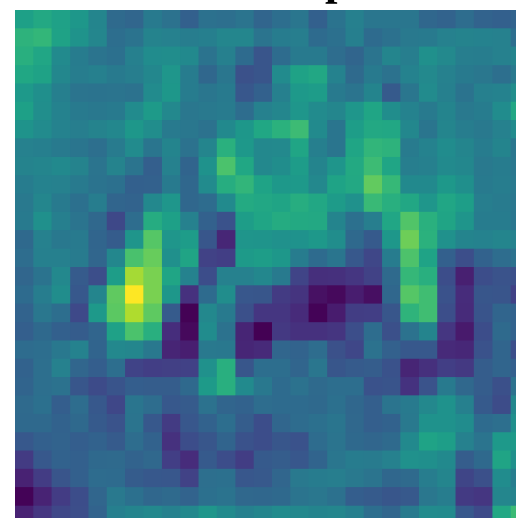
5x5 - map 3
