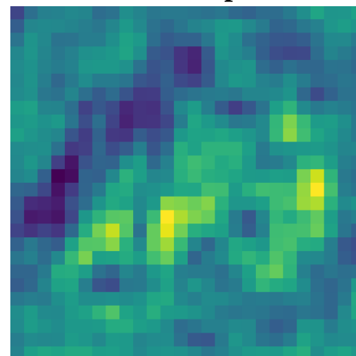
7x7 - map 3
