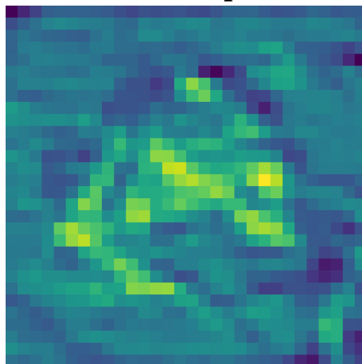
5x5 - map 2
