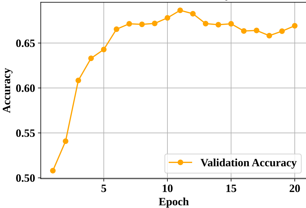
Validation Accuracy
