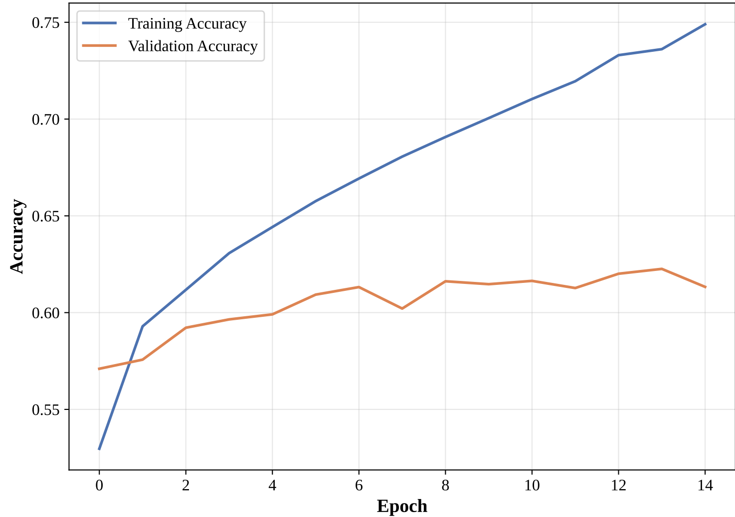
Figure 2: Training and Validation Accuracy
