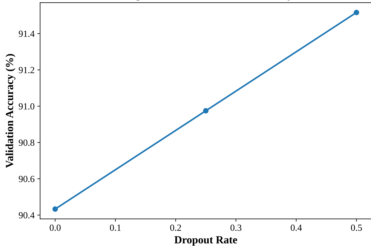
Dropout Rate vs. Validation Accuracy
