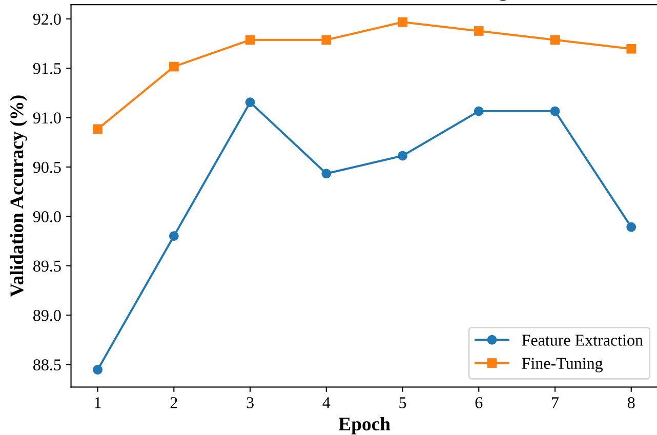
Feature Extraction vs. Fine-Tuning
