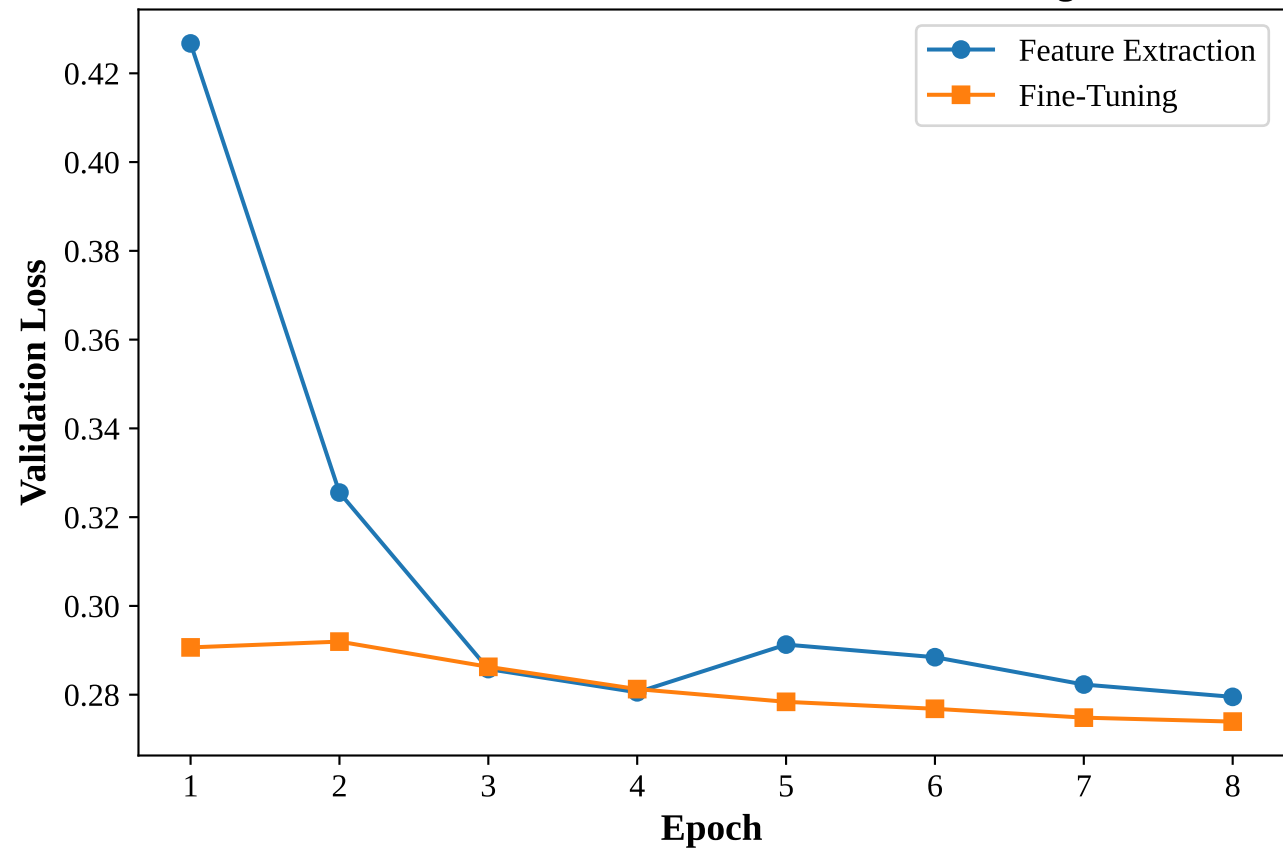
Validation Loss Before and After Fine-Tuning
