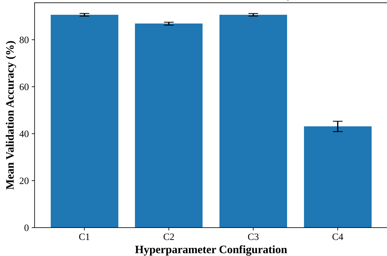
5-Fold Cross-Validation Accuracy
