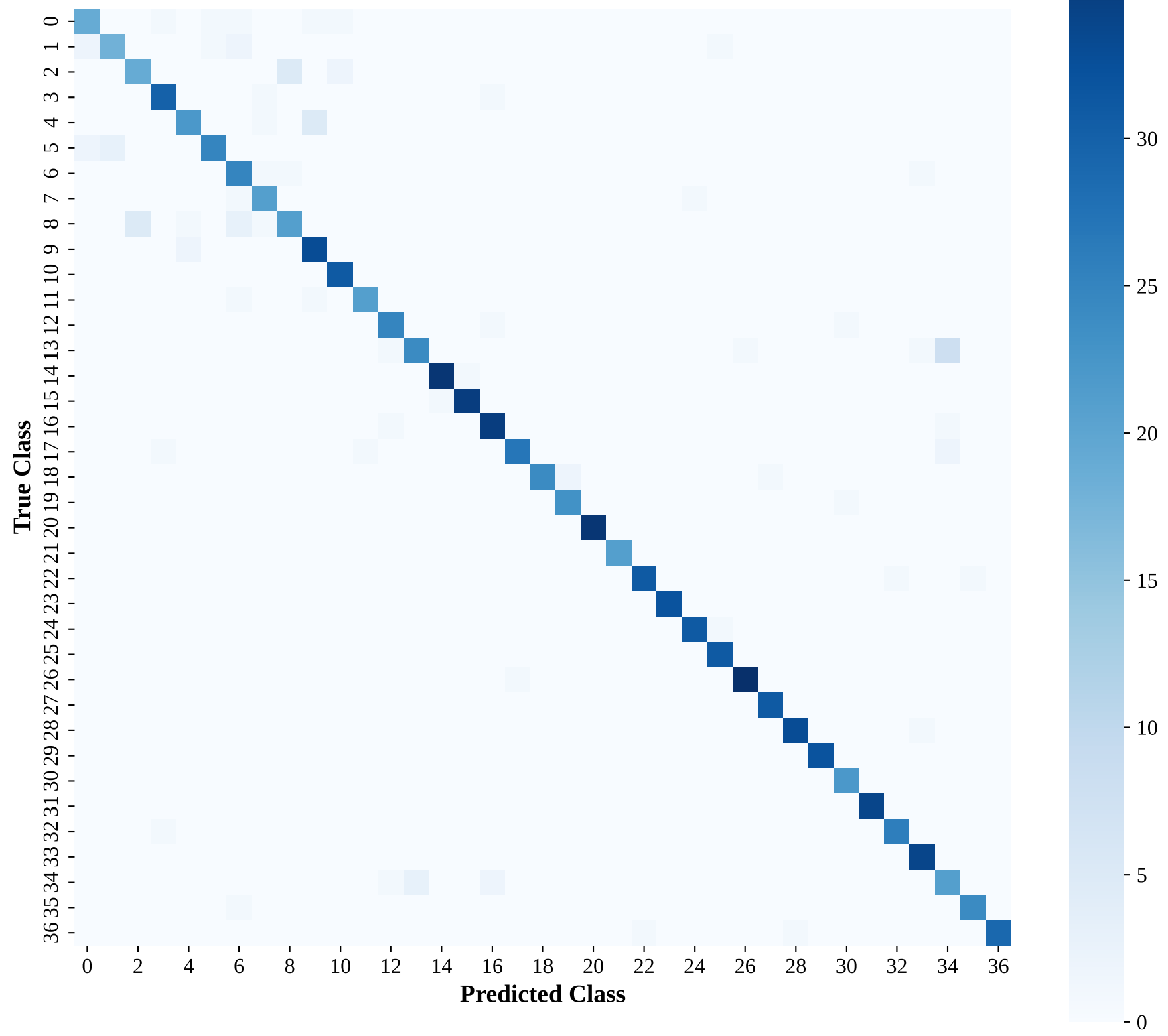
Confusion Matrix on Test Set
