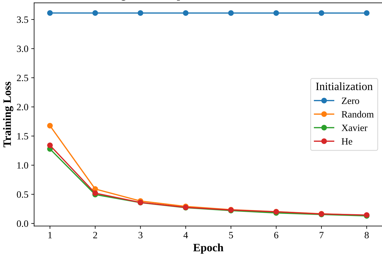
Training Loss vs. Epoch for Different Initializations
