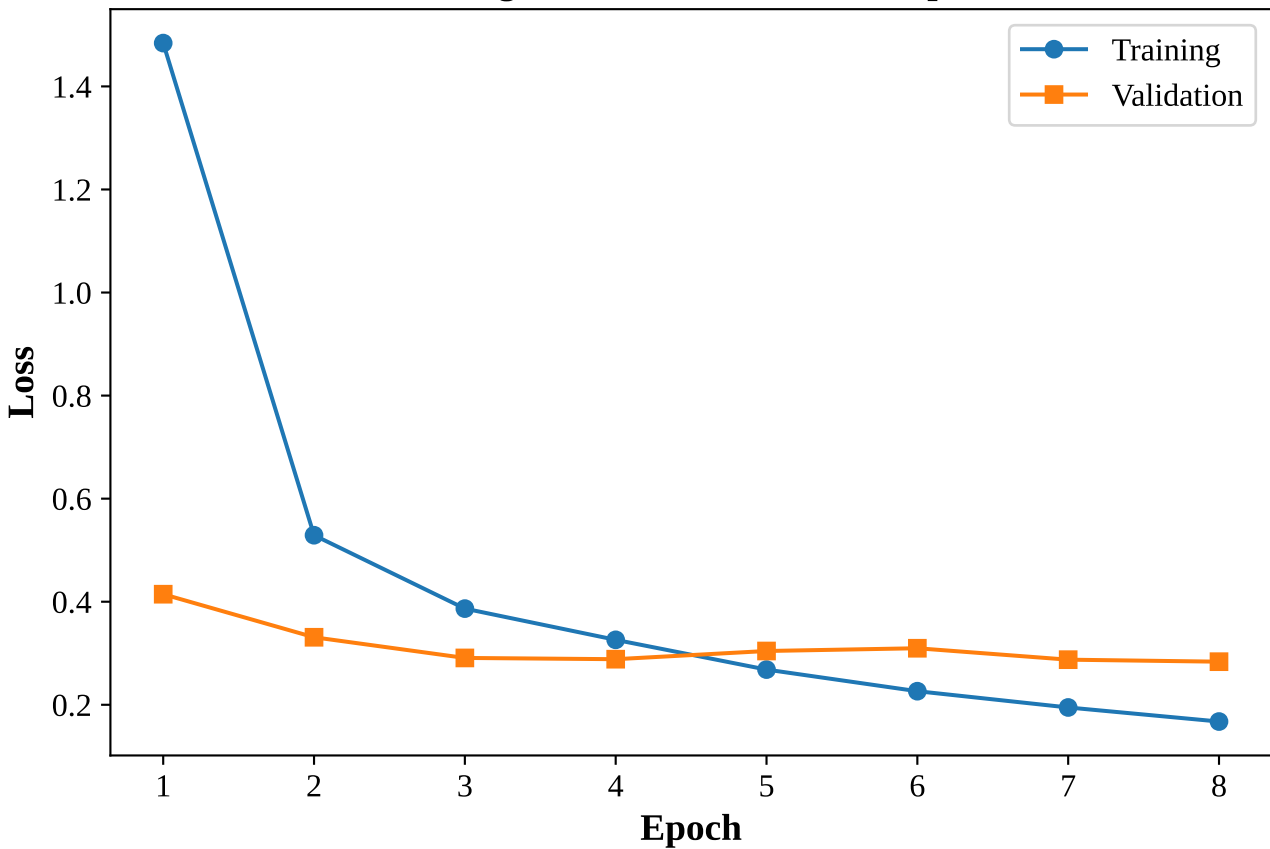
Training and Validation Loss vs. Epoch
