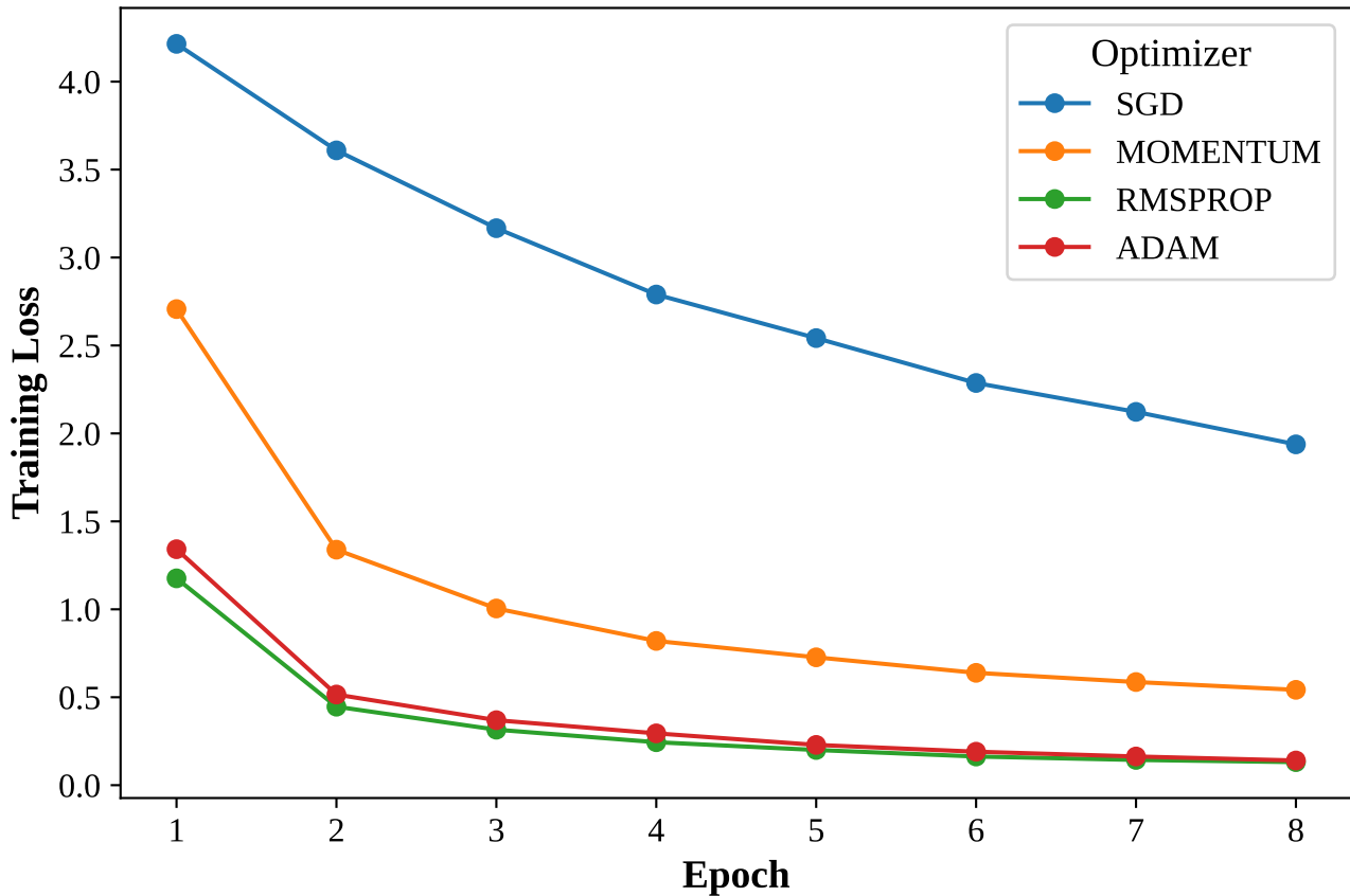
Training Loss vs. Epoch for Different Optimizers
