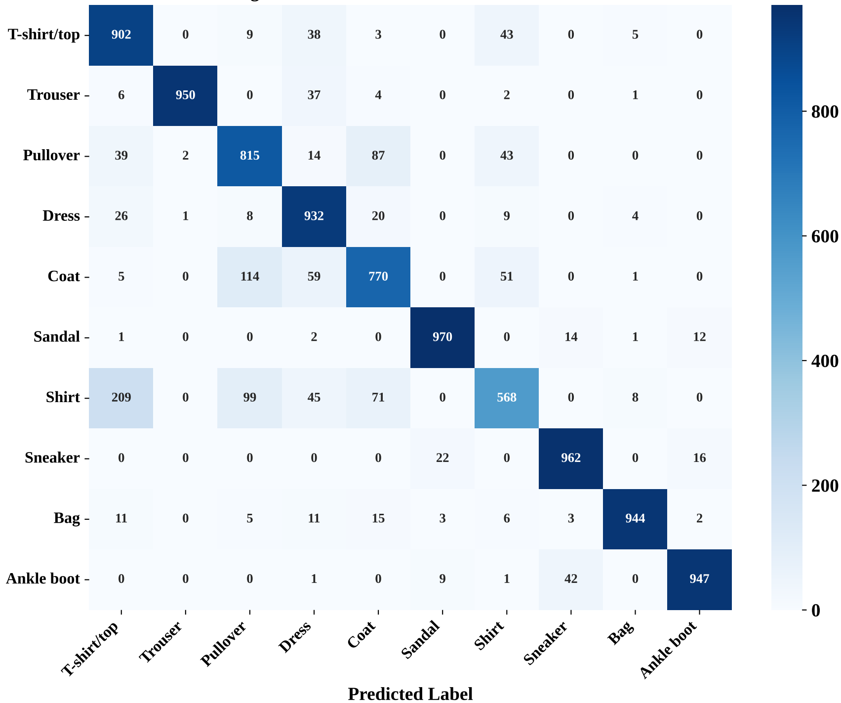
Figure 7: Confusion Matrix - Baseline Model
