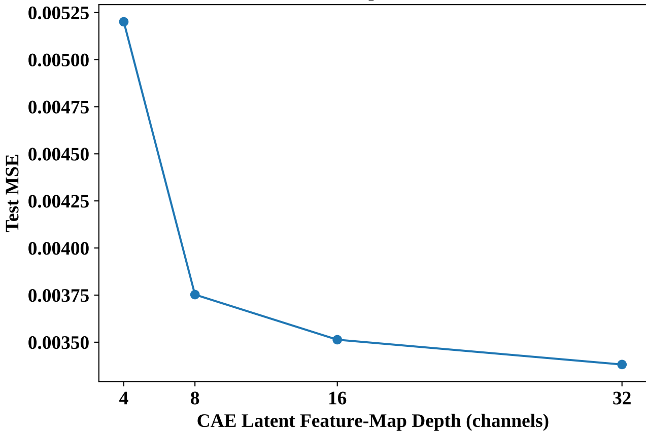
Exercise 1: CAE Latent Depth vs. Reconstruction MSE
