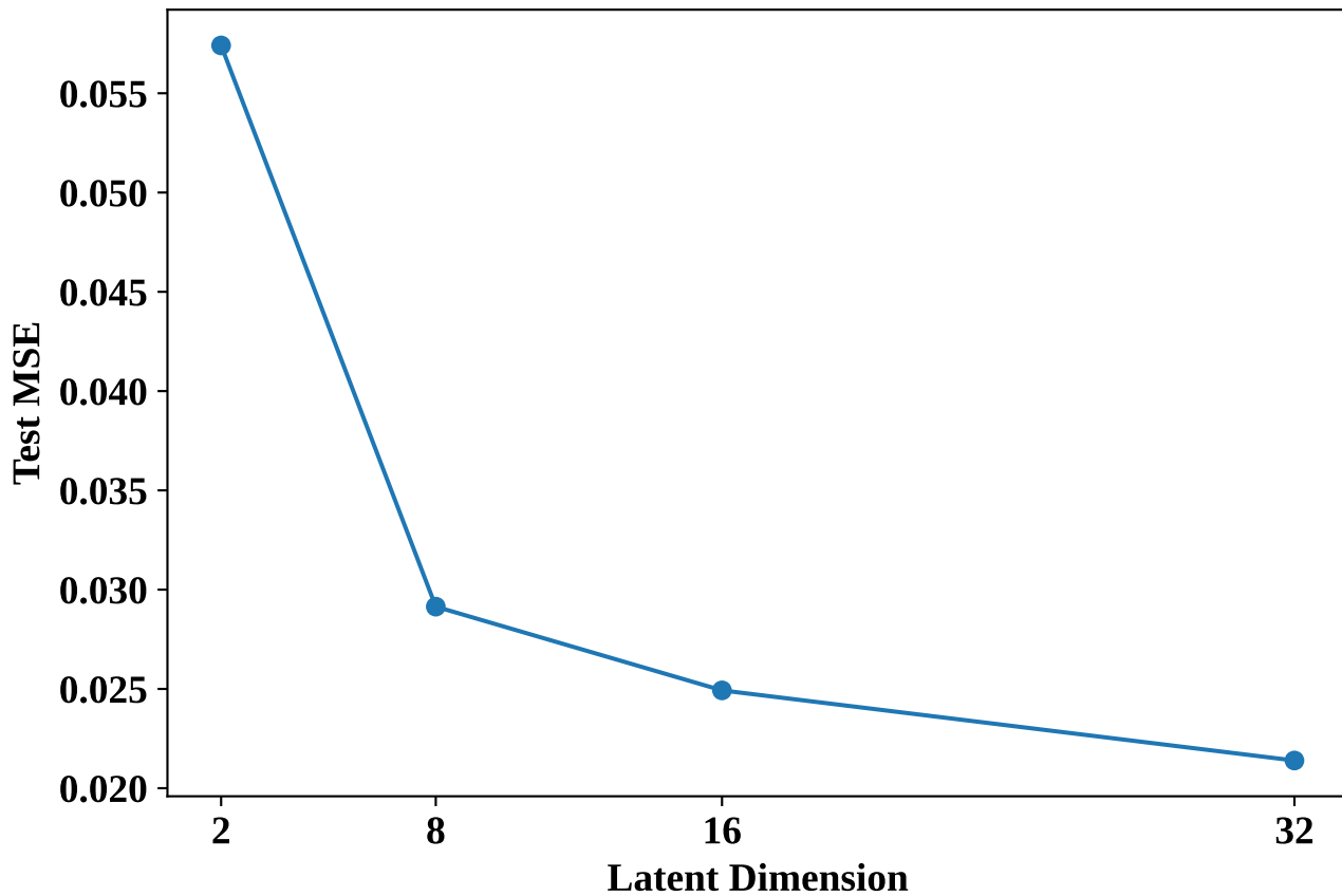
Plot 10: Latent Dimension vs. Reconstruction MSE
