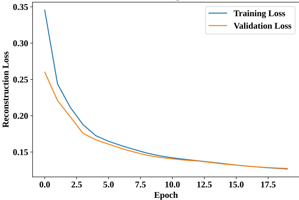
Plot 2: FC-AE Training/Validation Loss
