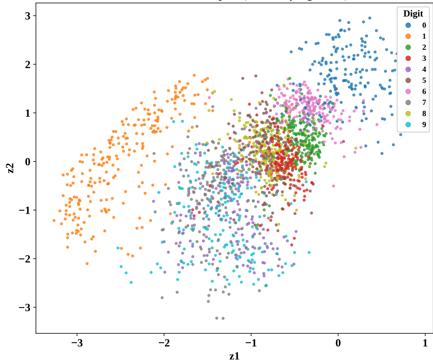
Plot 6: VAE Latent Space (colored by digit label)
