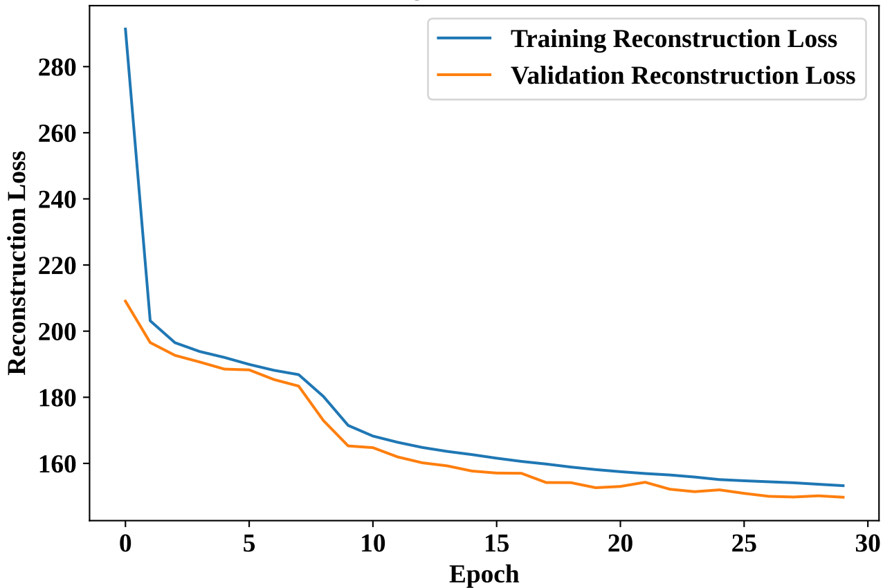
Plot 9: VAE Training/Validation Reconstruction Loss
