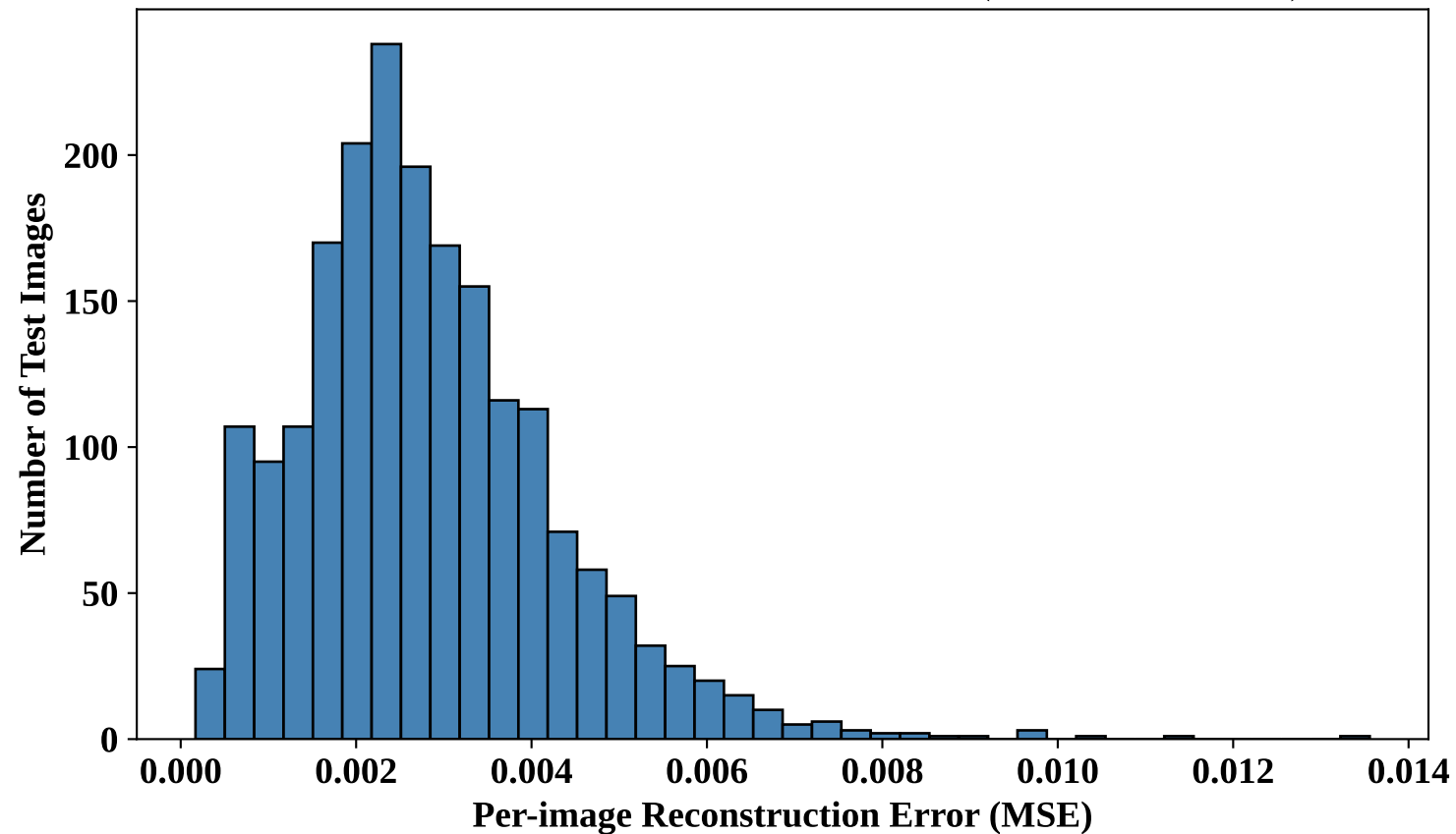
Plot 9: Distribution of Reconstruction Errors (Conv. Autoencoder)
