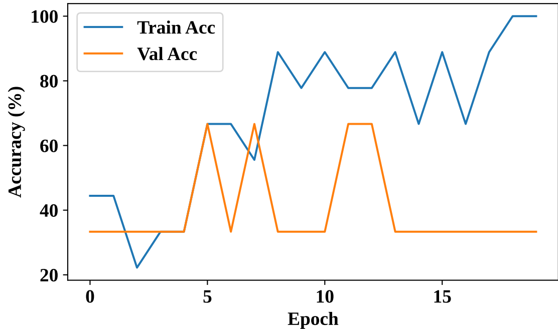
CNN_LSTM_video: Accuracy
