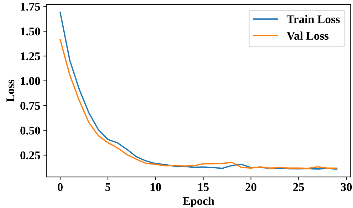
GRU: Loss
