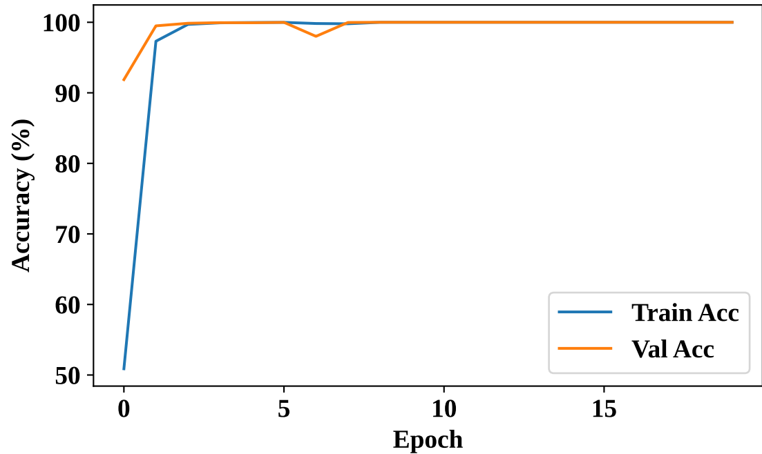
Seq2Seq_reversal: Accuracy
