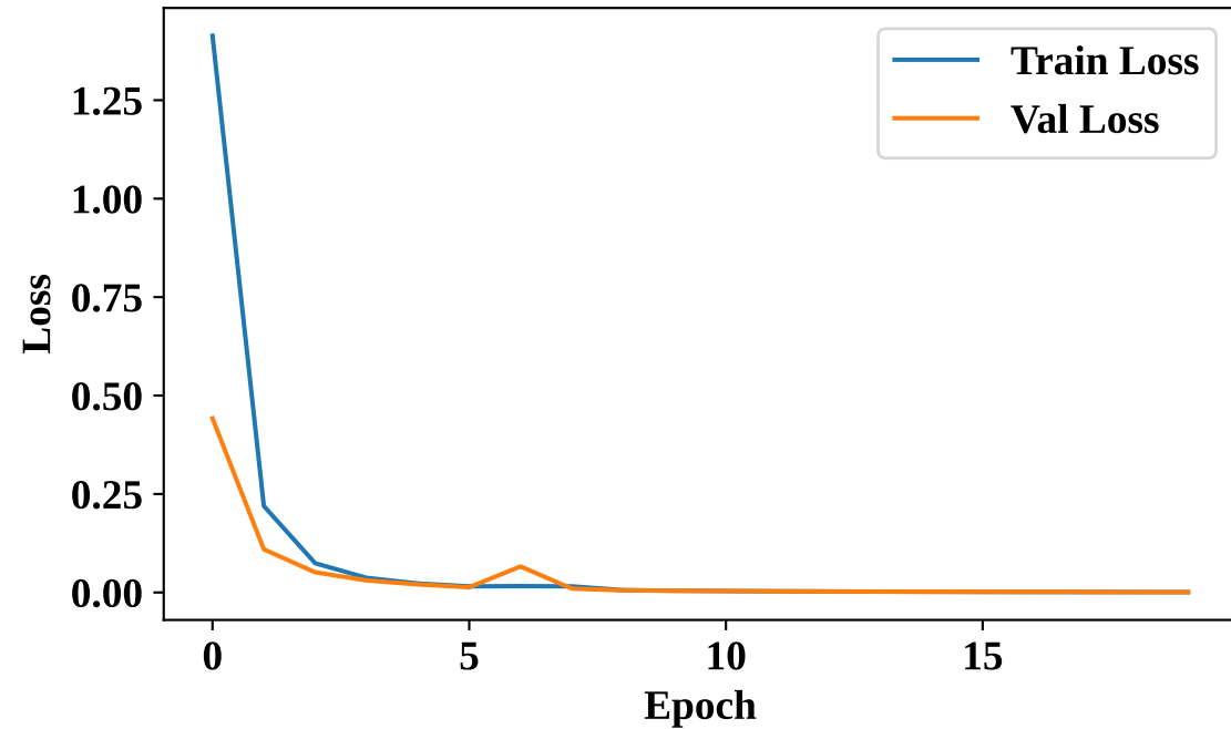
Seq2Seq_reversal: Loss
