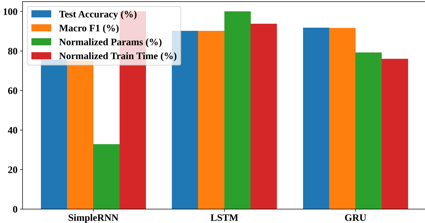
Plot 5: RNN vs LSTM vs GRU Comparison
