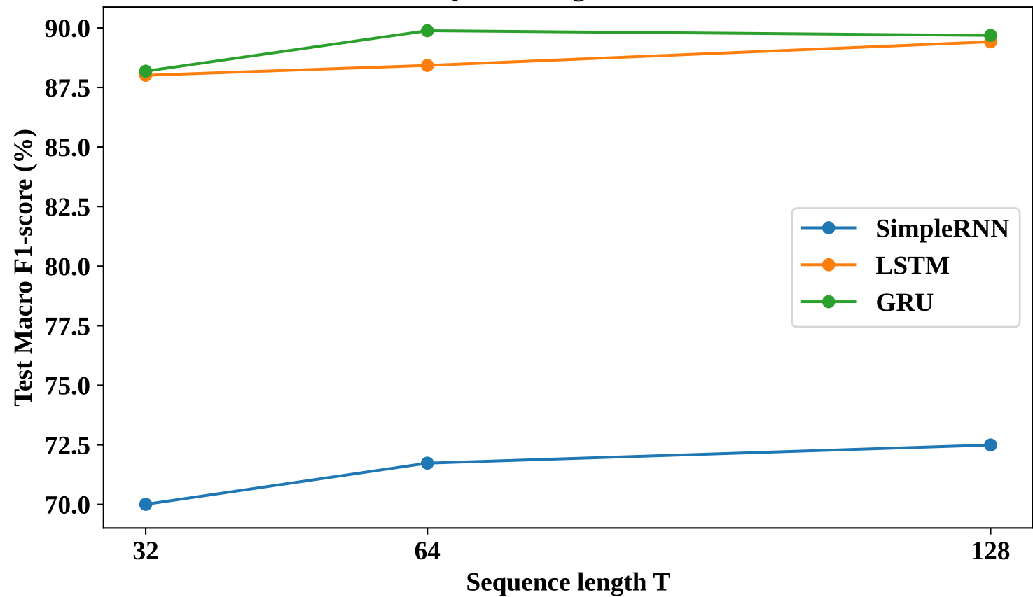
Plot 6: Sequence Length vs. Test F1-score
