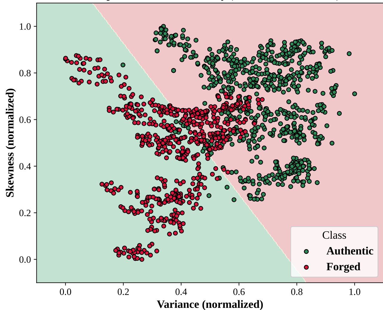
Perceptron Decision Boundary (Variance vs Skewness)
