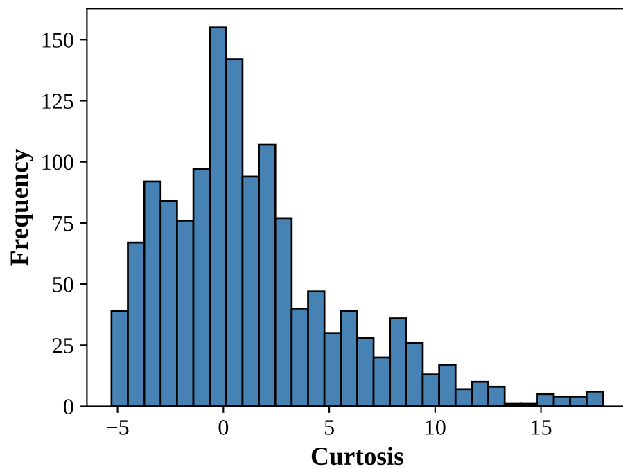
Distribution of Kurtosis
