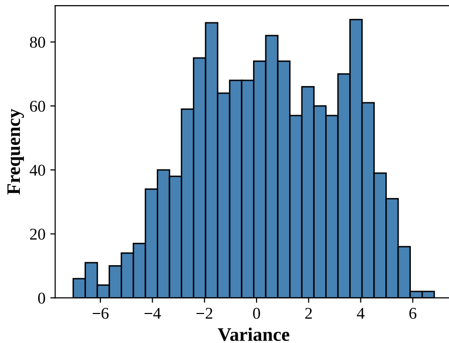
Distribution of Variance
