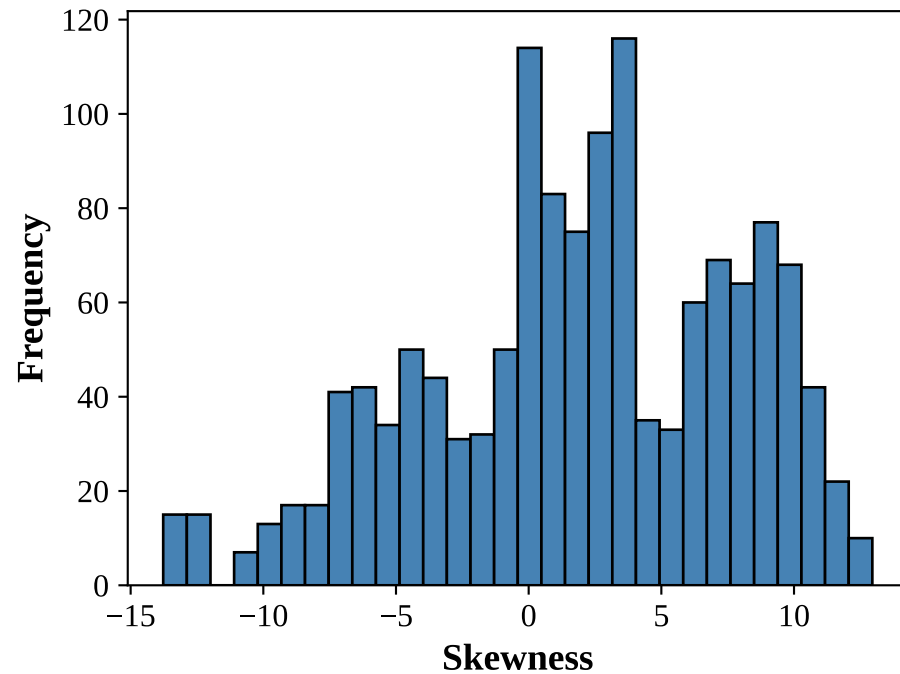
Distribution of Skewness
