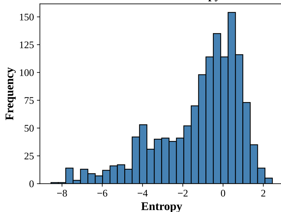
Distribution of Entropy
