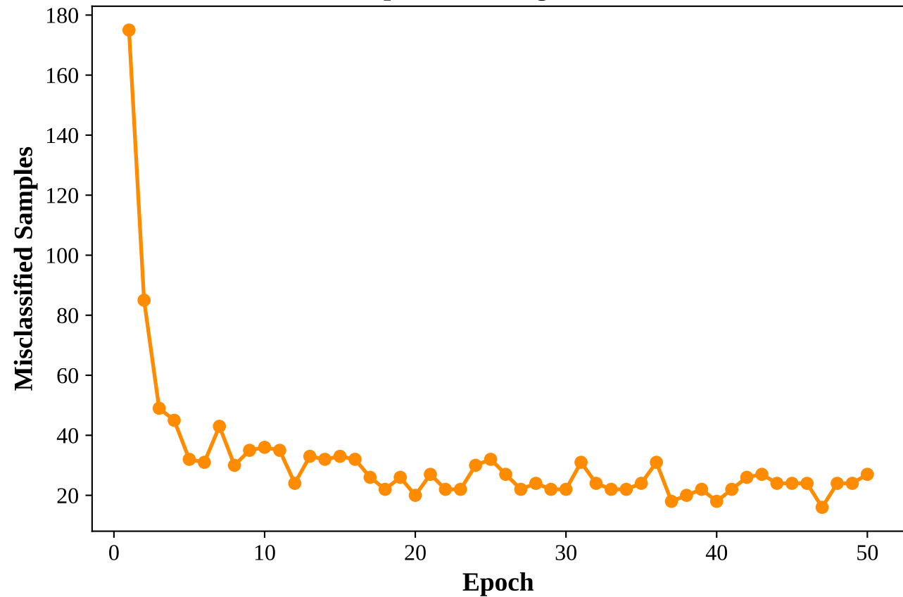
Perceptron Convergence Curve
