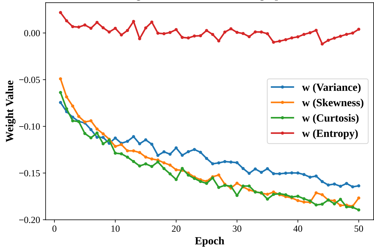
Weight Evolution over Training Epochs
