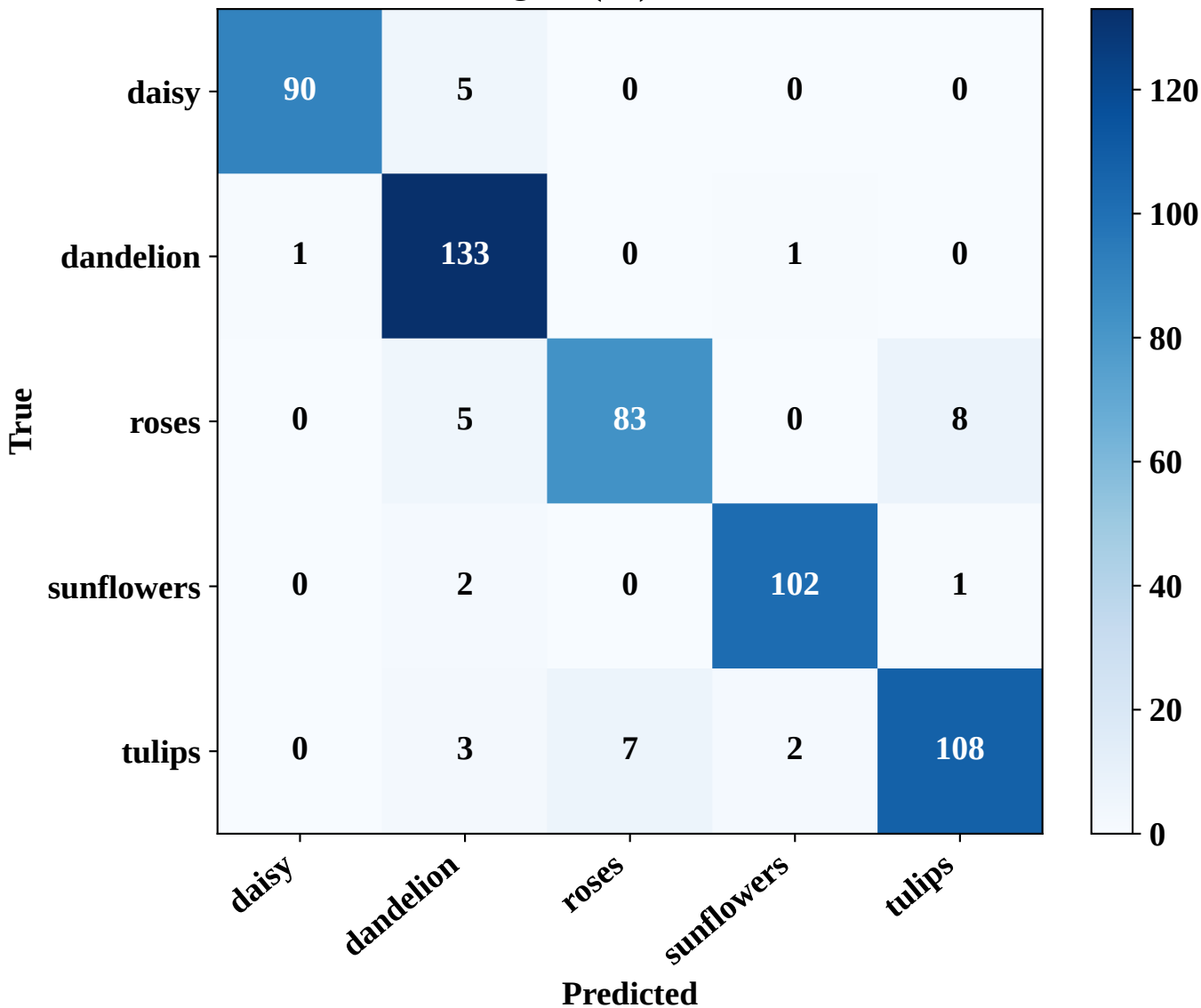
C+S @ P4 (P4) acc = 0.936
