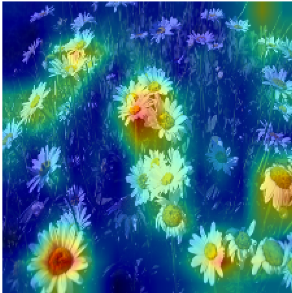
Feature map before attention
