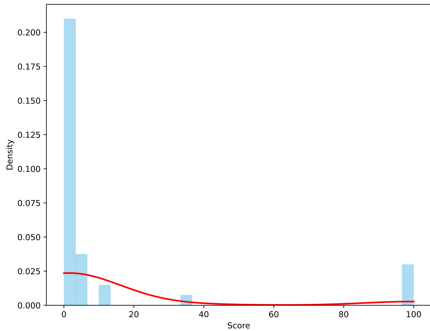
Score Distribution
