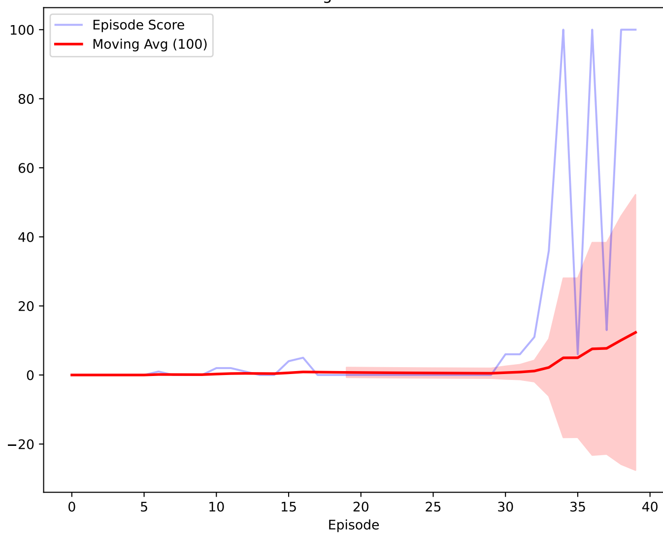
Epsilon Decay
