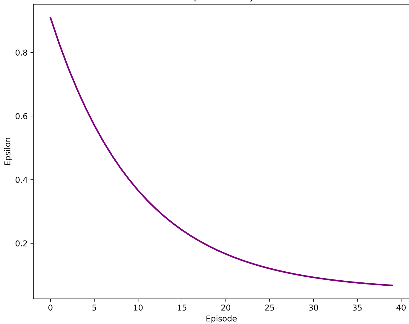
Epsilon Decay
