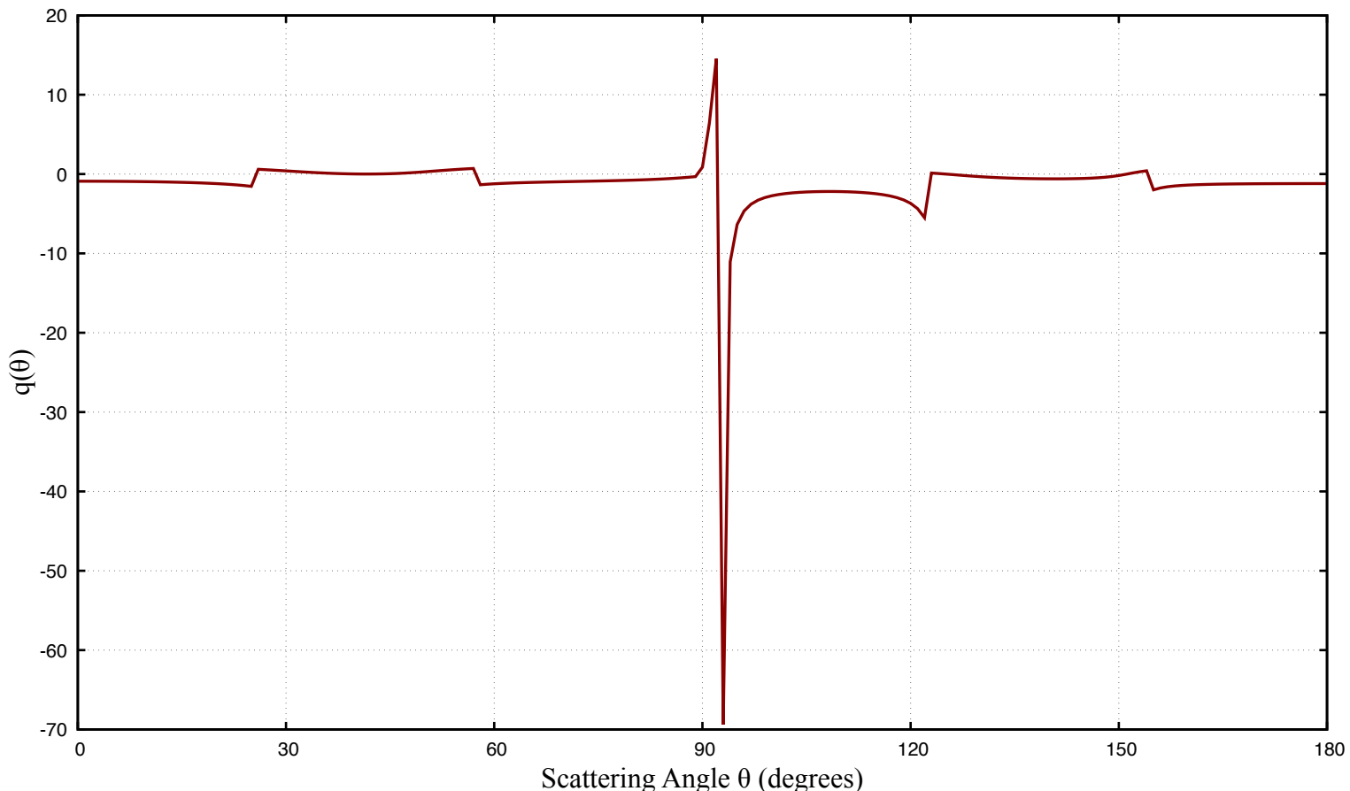
H+Xe: Angle-Dependent Fano q-parameter ( l=5 )
