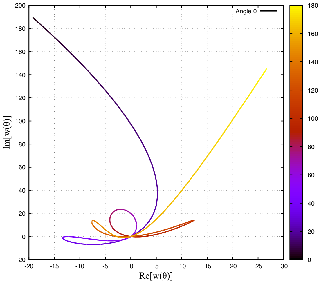
H+Xe: Complex w(\theta) Trajectory ( l=5 )
