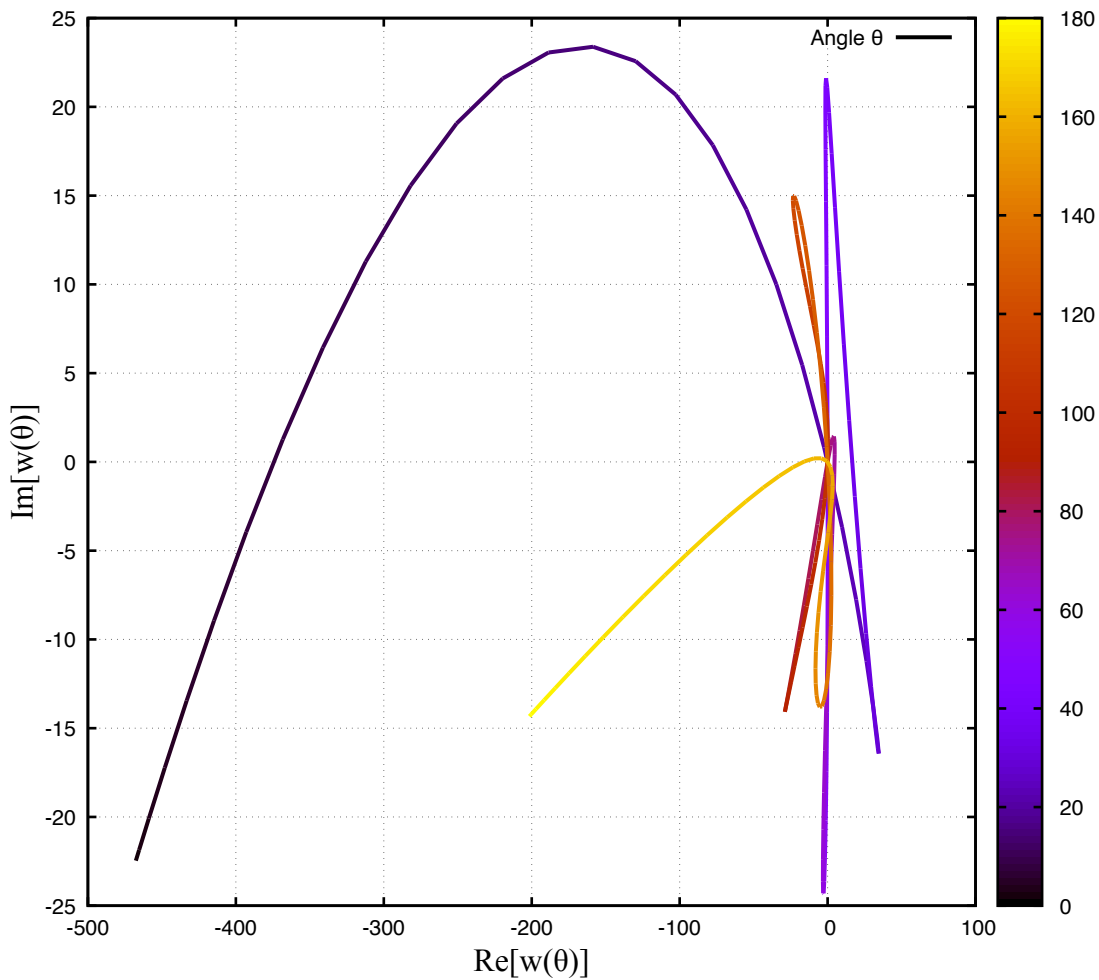
H+Xe: Complex w(\theta) Trajectory ( l=6 )
