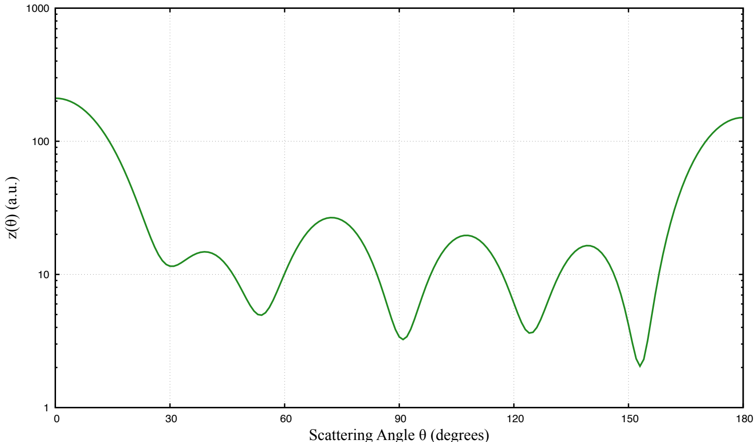
H+Xe: Background Factor z(\theta) ( l=5 )
