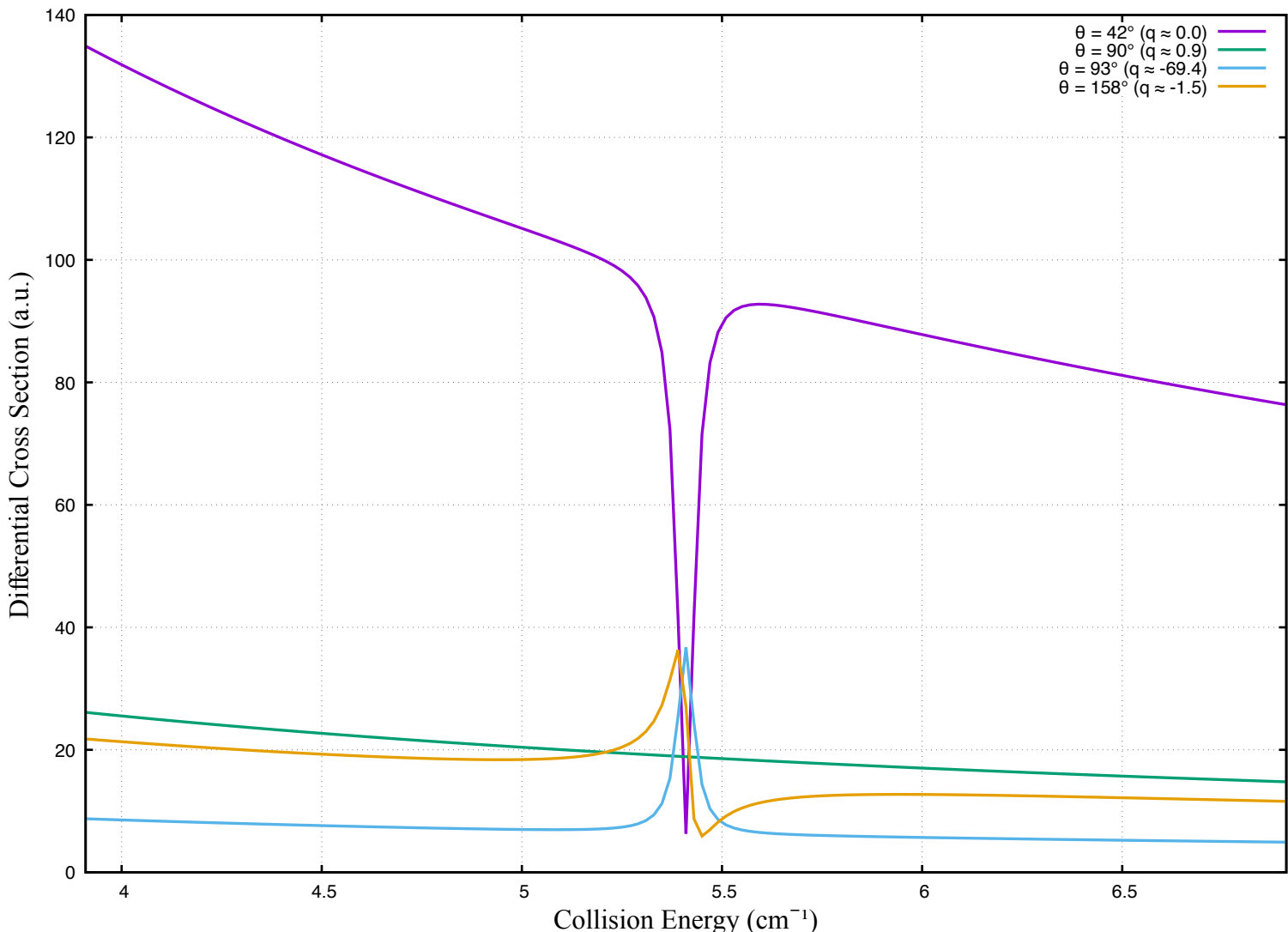
H+Xe: Archetypal Fano Resonance Profiles ( l=5 , E_r=5.41 \text{ cm}^{-1} )
