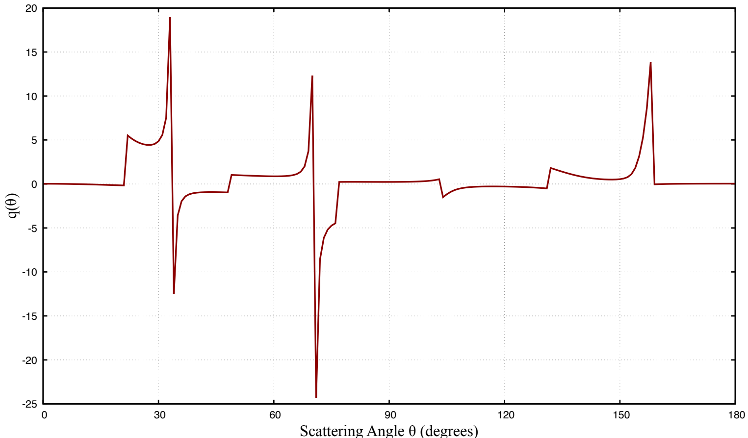
H+Xe: Angle-Dependent Fano q-parameter ( l=6 )
