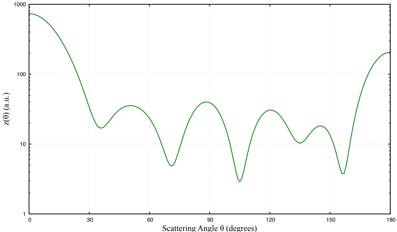
H+Xe: Background Factor z(\theta) ( l=6 )
